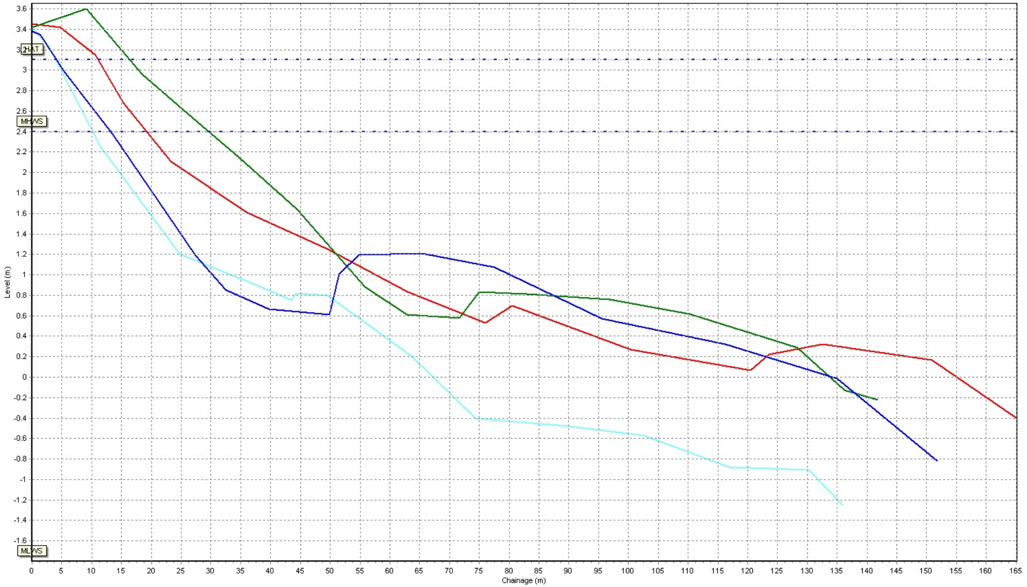
Beach Profiles: 1aWDC10
