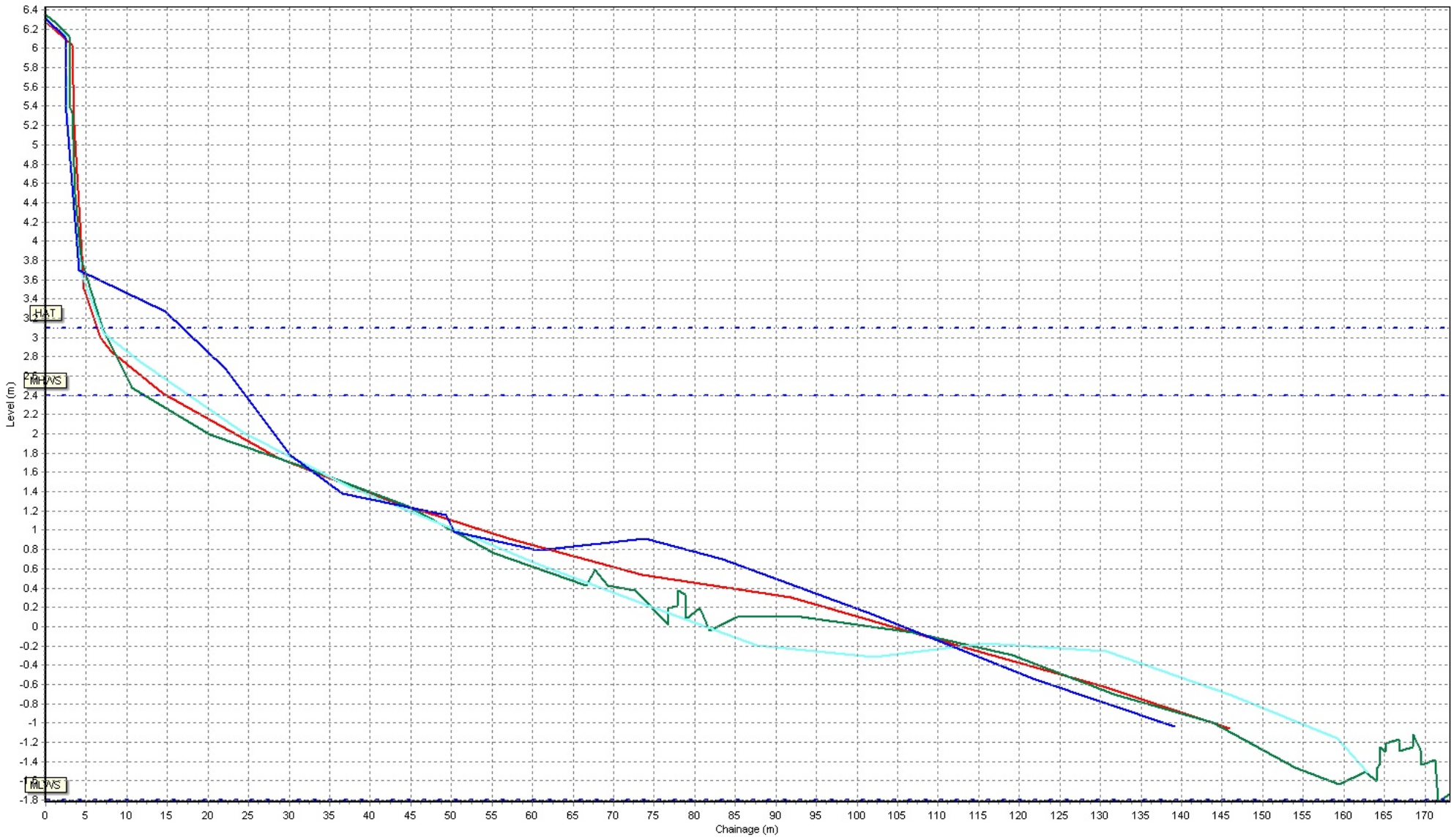
Beach Profiles: 1aWDC14
