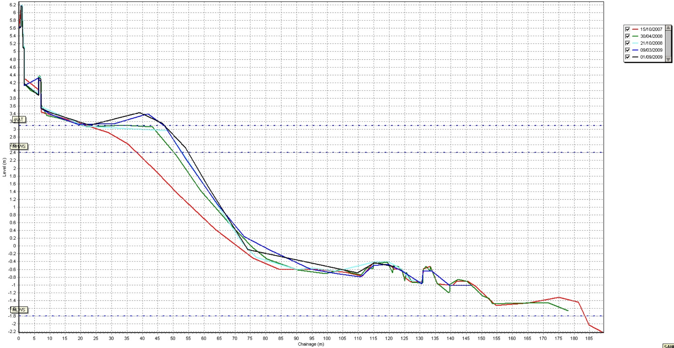
Beach Profiles: 1aWDC05A
