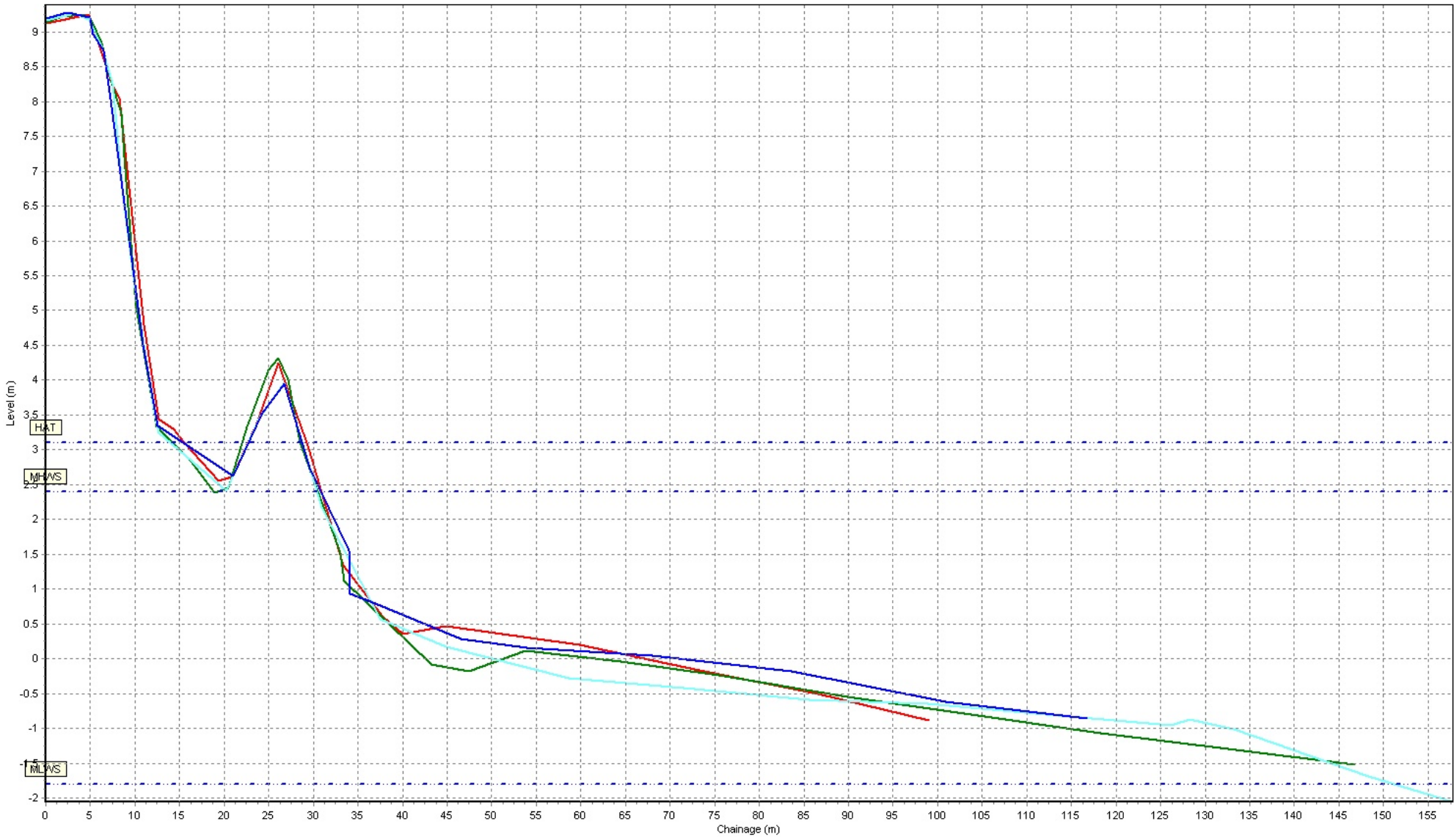
Beach Profiles: 1aWDC08
