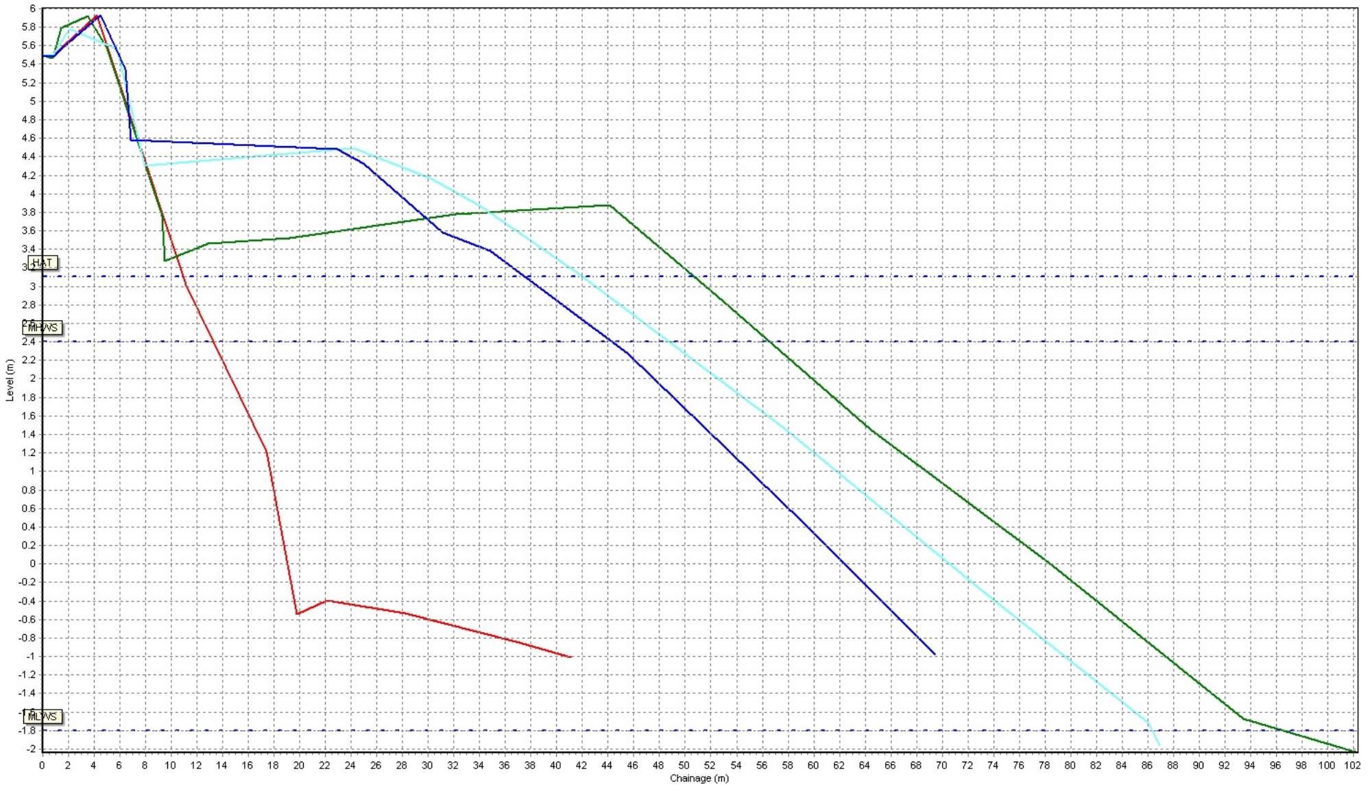
Beach Profiles: 1aWDC07
